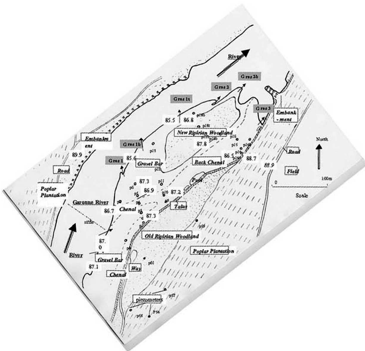
Fig. 1. General view of Garonne river meander near Monbéli, S.W. France. The nature of the land use is given in the framed white rectangles. Some elevations (in metres above sea level) are reported in smaller white rectangles to give an idea of the profile section of this field site. The possible water input (river water into groundwater, two before the riffle) and output (groundwater into the river water, six after the riffle, numbered in a grey rectangle) are indicated by black arrows. The figure is completed with the position of the numerous piezometers (black circles with numbers) used in this study.
